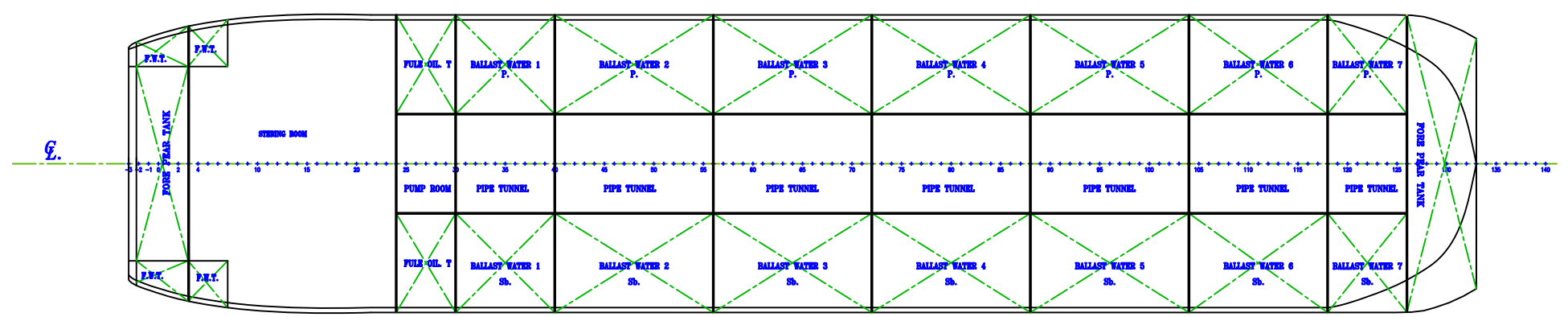
TANK TOP PLAN
