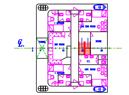
OFFICER DECK
